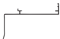
HS017 Special Subsill Ext Width 35mm
