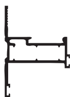
SF012 Awning Sash 53 X 36 suits SF041 stake
